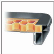
Hexagonal structure
