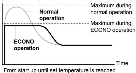
Running current and power consumption
