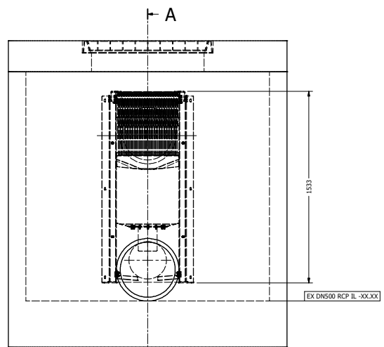
PLAN VIEW SCALE (DNS)
