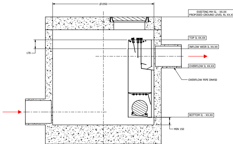
SECTION A-A SCALE (DNS)
