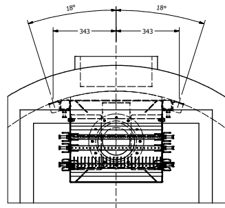
DETAIL A WALL FIXING LOCATION DETAIL ACCESS LID NOT SHOWN FOR CLARITY SCALE (DNS)
