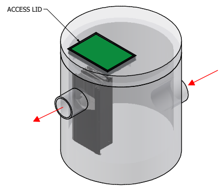
ISOMETRIC VIEW SCALE (DNS)
