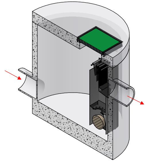
SECTION VIEW ISOMETRIC SCALE (DNS)
