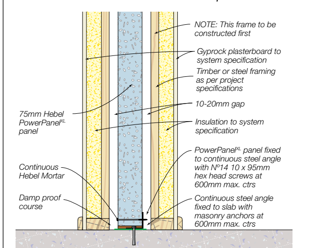
Detail 3.5 Base Connection - Option 2
