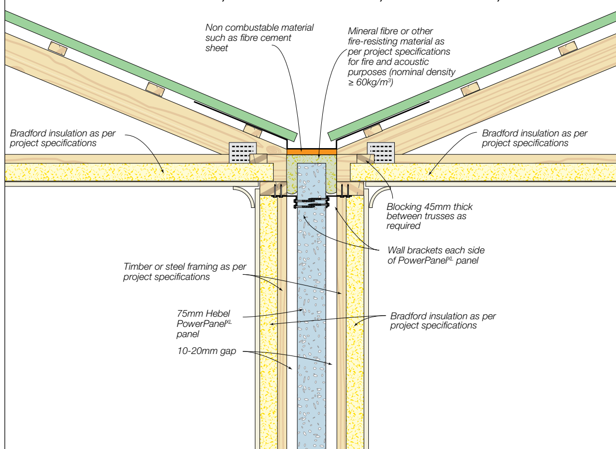
Detail 3.9 Roof Valley for PowerPanel XL Intertency Discontinuous Wall Systems
