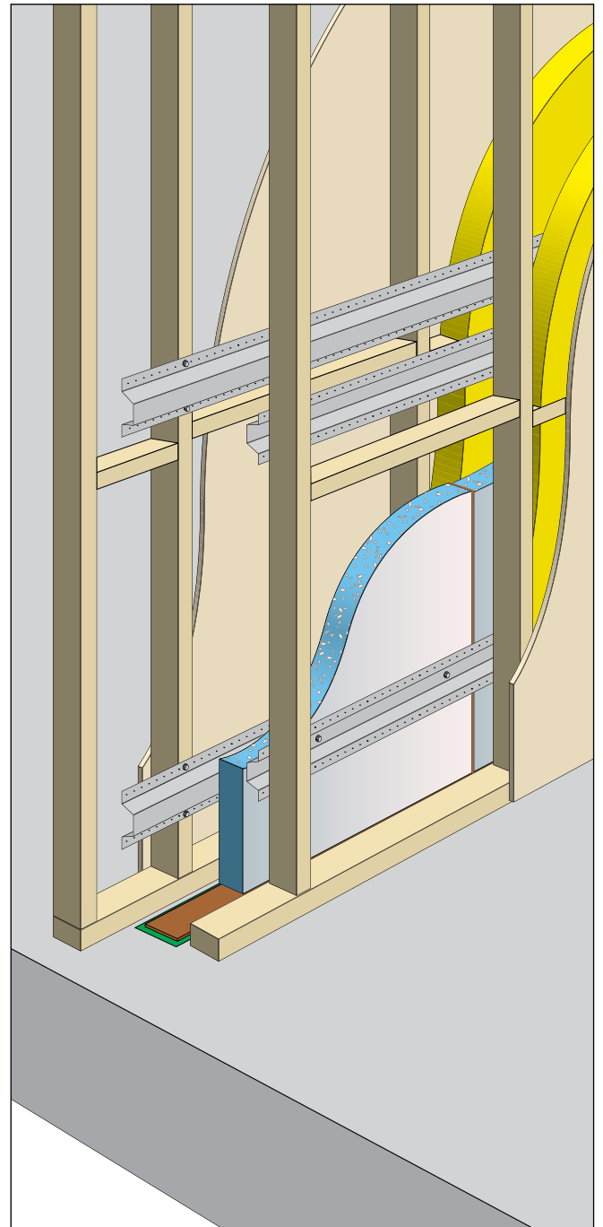
Detail 1.2 PowerPanel XL Intertenancy Non-discontinuous Wall Systems
