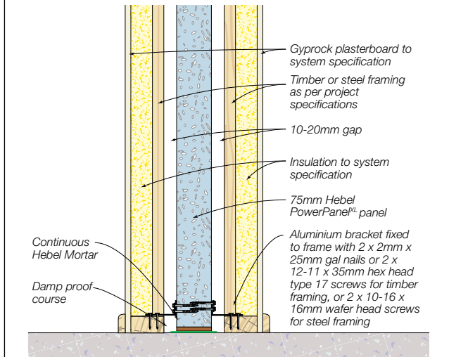
Detail 3.3 Base Connection - Option 1
