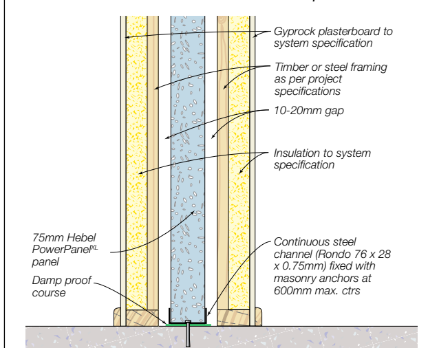
Detail 3.7 Base Connection - Option 3
