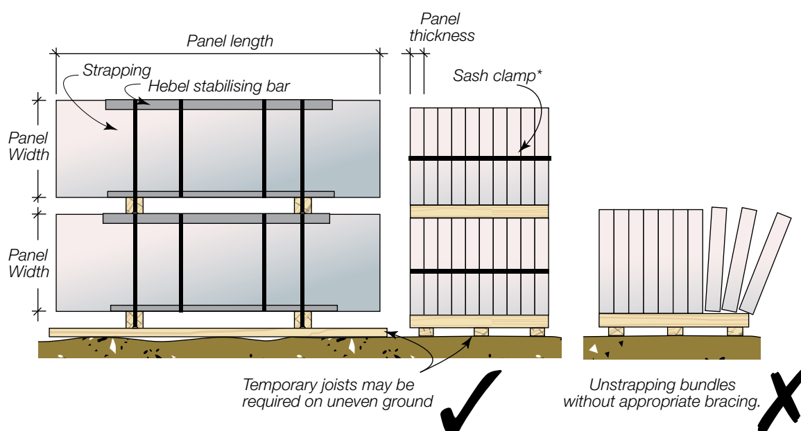
Fig. 4.1 Stacking Packs of Hebel PowerPanel XL
