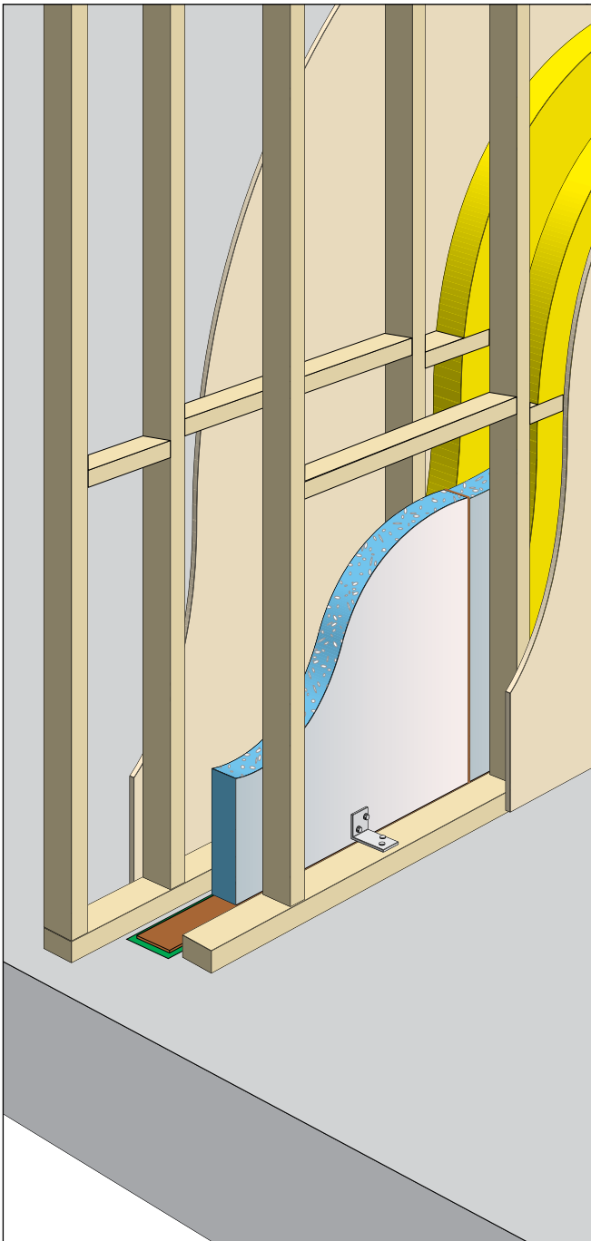
Detail 1.1 PowerPanel XL Intertenancy Discontinuous Wall Systems
