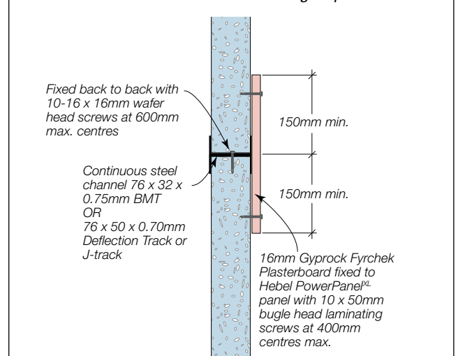
Detail 3.6 Horizontal Joint Fixing - Option 2
