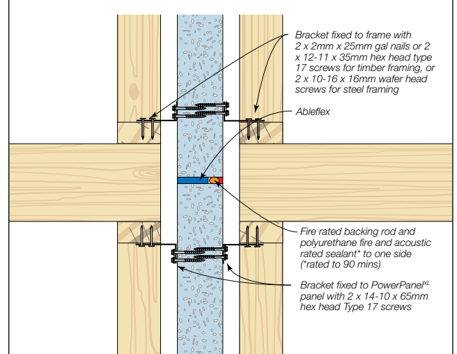
Detail 3.4 Horizontal Joint Fixing - Option 1
