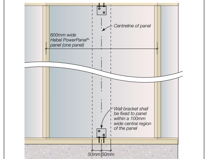
Detail 3.8 Bracket Fixing
