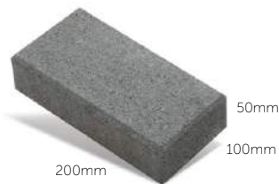
Havenbrick® 50
