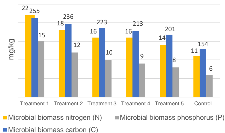
Figure 8. Increase in microbial C, N and P as a result of various treatments.
